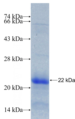
Recombinant Mouse Cdkn1a SDS-PAGE
