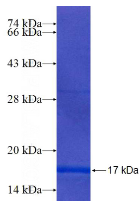
Recombinant Human DYNLRB1 SDS-PAGE
