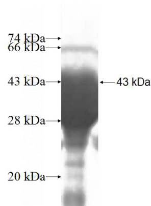
Recombinant Human NAGK SDS-PAGE
