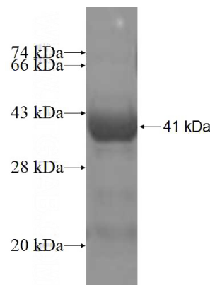
Recombinant Human DHDH SDS-PAGE
