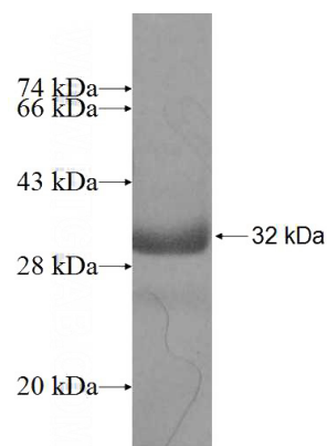
Recombinant Human NT5C3L SDS-PAGE
