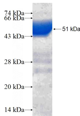
Recombinant Human NAPSA SDS-PAGE
