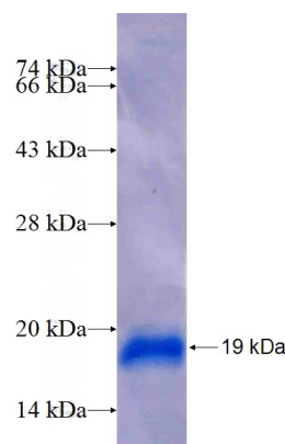
Recombinant Human NR1H4 SDS-PAGE
