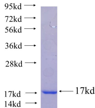
Recombinant human TMC8 SDS-PAGE
