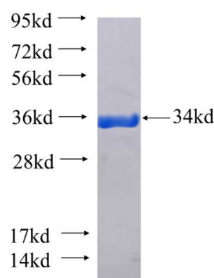
Recombinant human SLC13A3 SDS-PAGE
