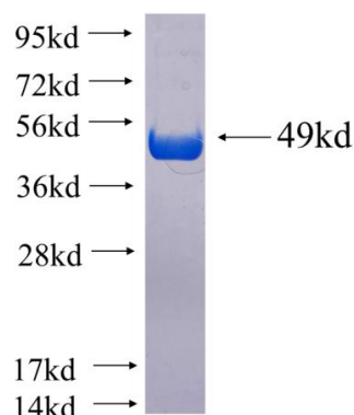
Recombinant human RP11-529I10.4 SDS-PAGE
