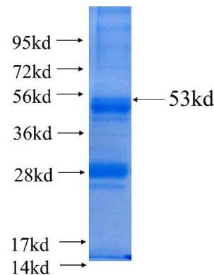
Recombinant human RND3(Full length) SDS-PAGE
