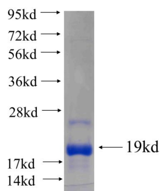
Recombinant human PUM1 SDS-PAGE
