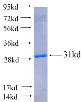
Recombinant human NPY5R SDS-PAGE
