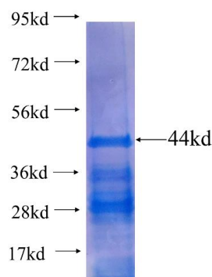
Recombinant human FAM129A SDS-PAGE
