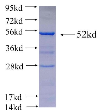
Recombinant human EPB49(Full length) SDS-PAGE
