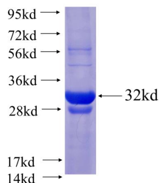
Recombinant human CAPZB SDS-PAGE
