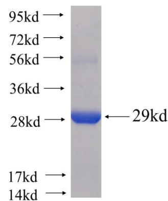
Recombinant human ARFRP1(Full length) SDS-PAGE
