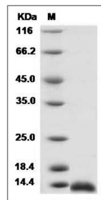
Rat CCL3 / Mip1a Protein SDS-PAGE
