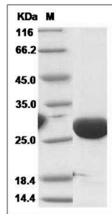
Human Phosphomannomutase 2 / PMM2 / CDG1 Protein (His Tag) SDS-PAGE
