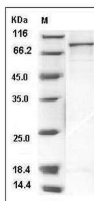
Human CAMKV Protein (His & GST Tag) SDS-PAGE
