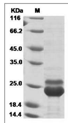
Human K-Ras / K-Ras (12 Asp) Protein (His Tag) SDS-PAGE
