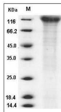
Human CD96 Protein (His Tag) SDS-PAGE
