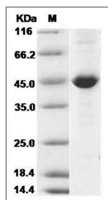
Human CKB / Creatine kinase B type Protein (His Tag) SDS-PAGE
