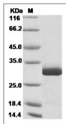
Human GSTM5 Protein (His Tag) SDS-PAGE
