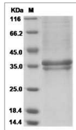
AGRP protein SDS-PAGE
