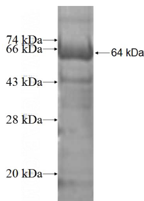
Recombinant Human VRK2 SDS-PAGE
