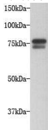
Fig1: Western blot analysis on HeLa cell lysates using anti-GOLGA5 Mouse mAb (Cat. # 176644#).
