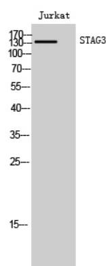
Fig1:: Western Blot analysis of Jurkat cells using STAG3 Polyclonal Antibody cells nucleus extracted by Minute TM Cytoplasmic and Nuclear Fractionation kit (SC-003, Invent biotech, MN, USA).
