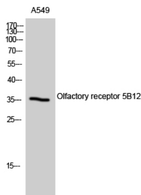
Fig1:: Western Blot analysis of A549 cells using Olfactory receptor 5B12 Polyclonal Antibody
