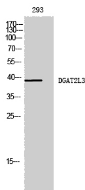
Fig1.; Western Blot analysis of 293 cells using DGAT2L3 Polyclonal Antibody diluted at 1: 1000
