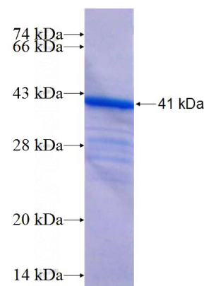
Recombinant Human XAB2 SDS-PAGE
