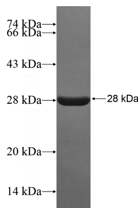
Recombinant Human MAP1B SDS-PAGE
