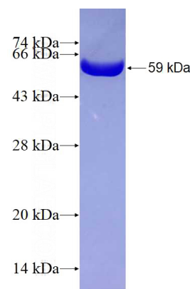
Recombinant Human FAK SDS-PAGE
