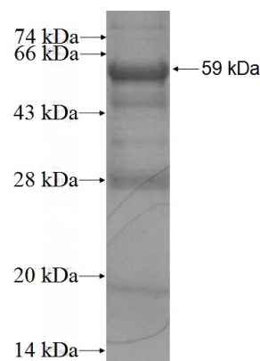
Recombinant Human RPA1 SDS-PAGE
