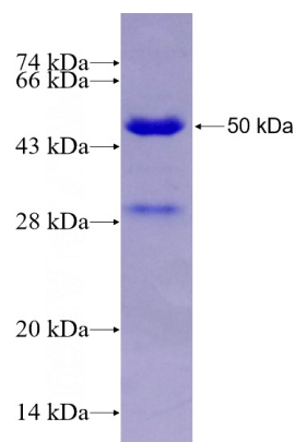
Recombinant Human SOX6 SDS-PAGE
