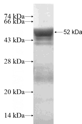
Recombinant Human SPAST SDS-PAGE
