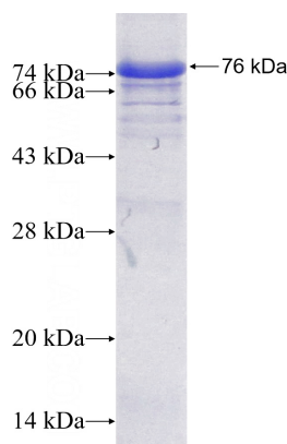
Recombinant Human Tubulin-Alpha SDS-PAGE
