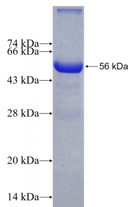
Recombinant Human NNMT SDS-PAGE
