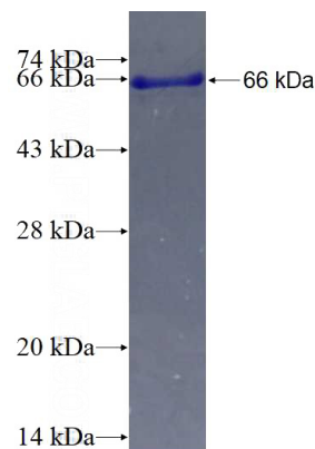
Recombinant Human HOMER1 SDS-PAGE
