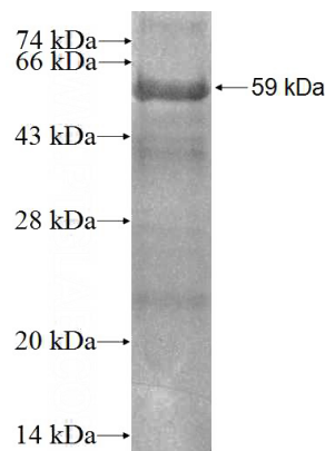
Recombinant Human GNB3 SDS-PAGE
