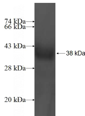
Recombinant Human POLR3K SDS-PAGE
