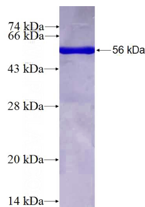
Recombinant Human GNPDA1 SDS-PAGE
