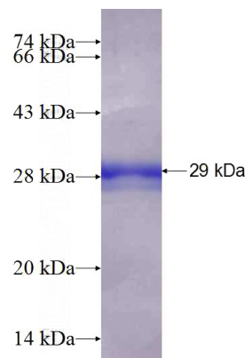
Recombinant Human FXN SDS-PAGE
