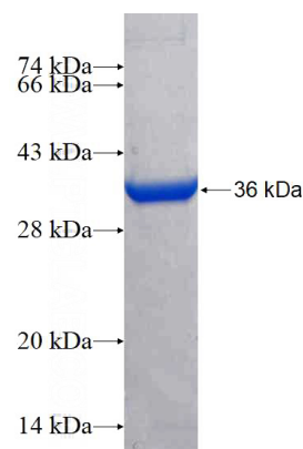
Recombinant Human OAS3 SDS-PAGE
