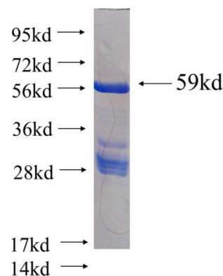
Recombinant human ZO1 SDS-PAGE
