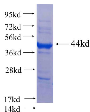
Recombinant human TDO2 SDS-PAGE
