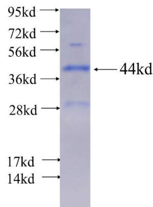
Recombinant human SHOC2 SDS-PAGE
