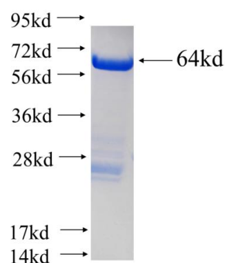
Recombinant human PDIA3 SDS-PAGE
