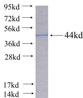
Recombinant human PDE5A SDS-PAGE
