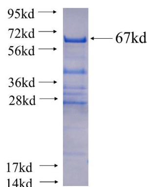
Recombinant human NFE2(Full length) SDS-PAGE
